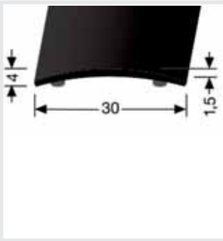
Transition moulding Type 438 Colour black
