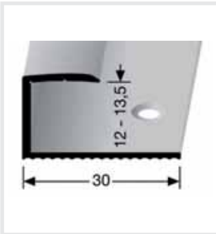
Joint moulding for Parquet Type 196
