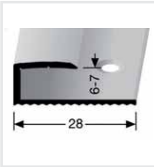
Joint moulding for Laminate Floors Type 192
