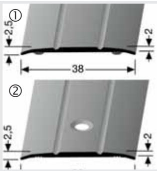
Transition moulding Type 438 Colour silver
