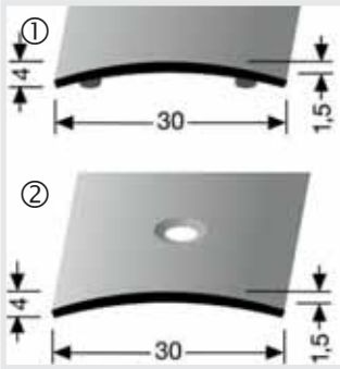
Transition moulding Type 459 Colour silver
