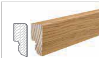
Skirtings without recess, veneered, matt-finished, 16x40 mm, cube
