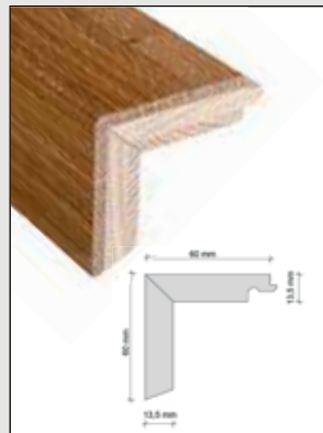
Stair nosing with connection on one side
