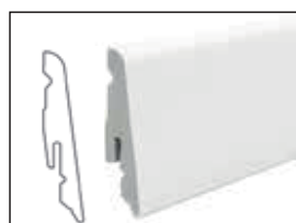
Stick-on skirtings PS foam, waterproof, suitable for damp rooms, 13.5x58 mm
